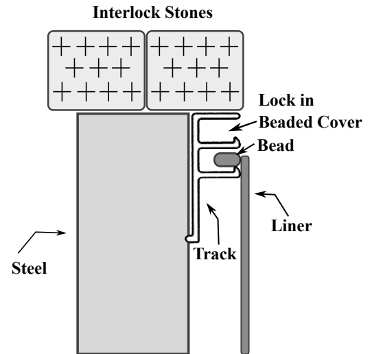
Double Track Side Mount Track
