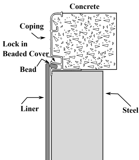
Double Track Flex Coping
