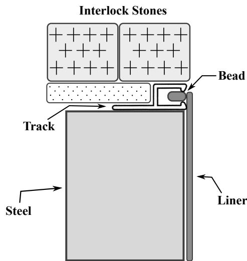
Single Track Top Mount Track
