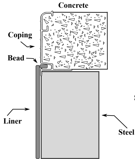
Single Track Flex Coping
