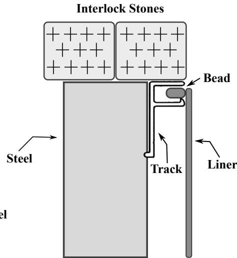
Single Track Side Mount Track
