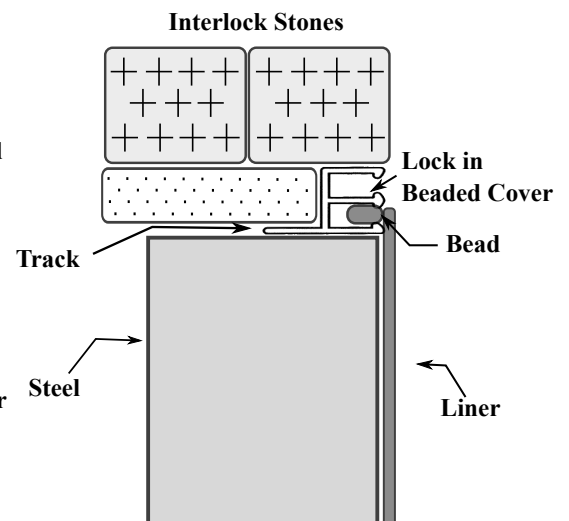
Double Track Top Mount Track
